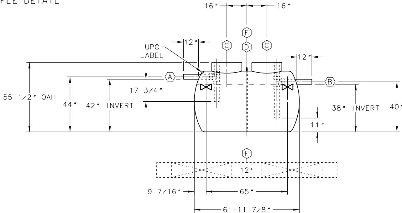
BAFFLE DETAIL
